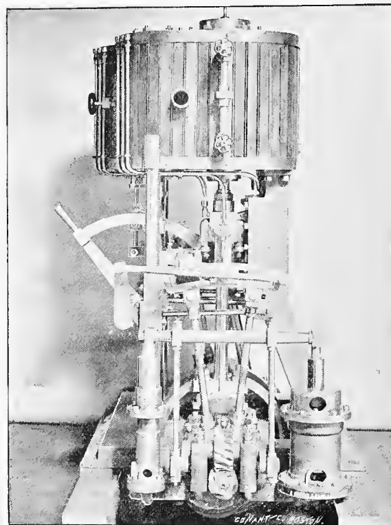
COMPOUND YACHT ENGINE, WITH AIR AND FEED-PUMP ATTACHED.—Designed and Built by the Edward S. Clark Co., Boston, Mass.
